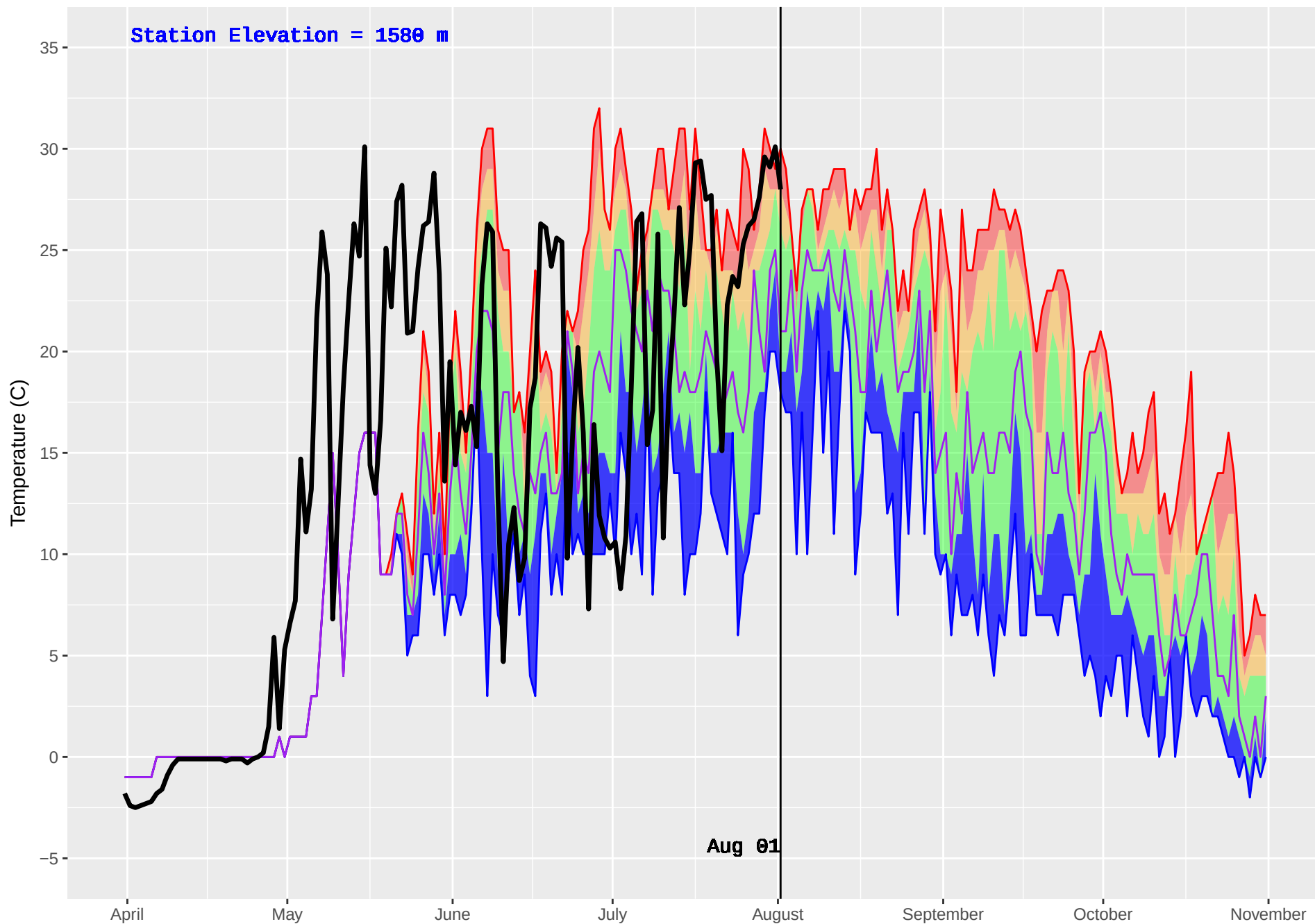
RORY CREEK (1092) : Historical (2010–2016) and Current (2018) Daily Temperature
