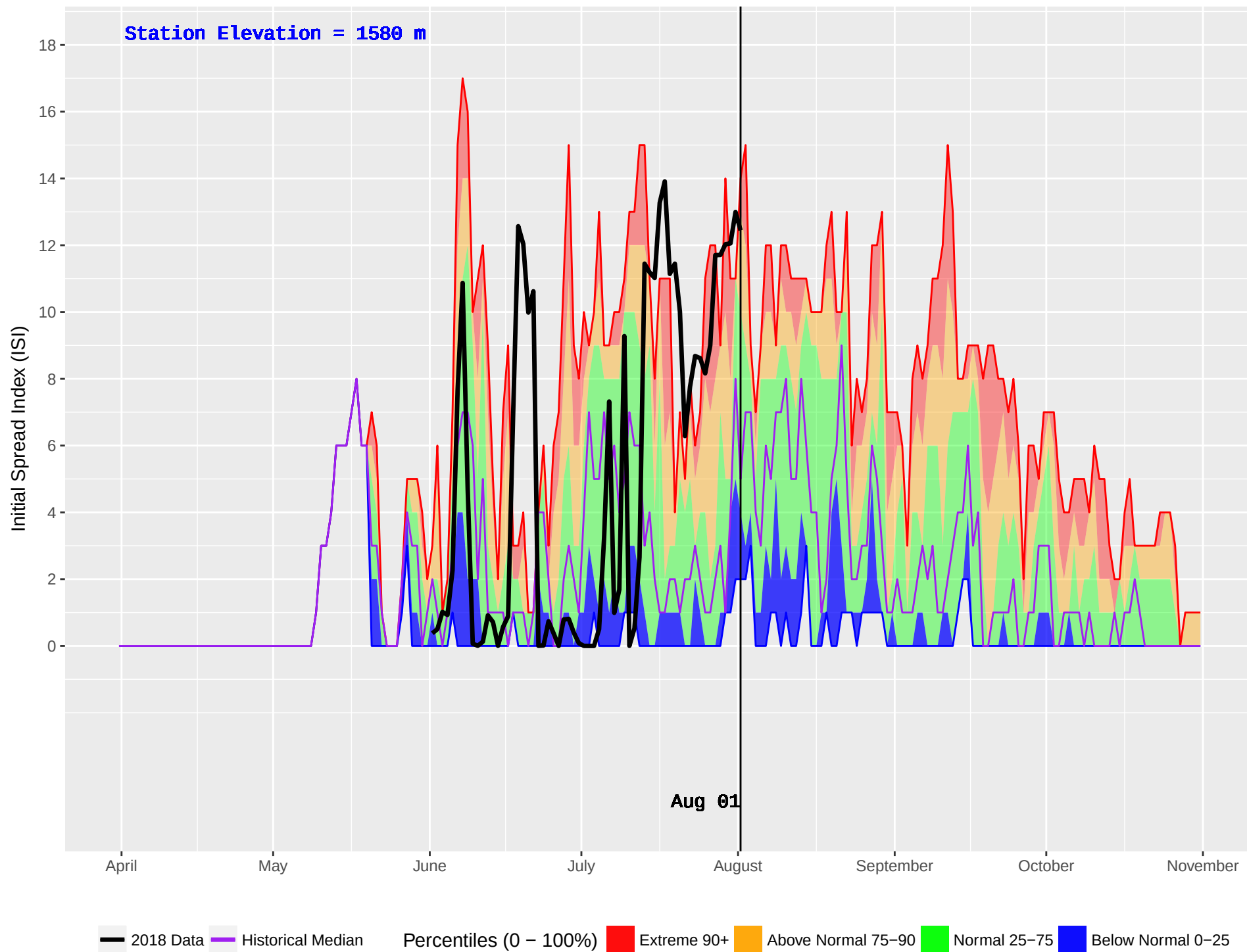
RORY CREEK (1092) : Historical (2010–2016) and Current (2018) Daily Initial Spread Index (ISI)
