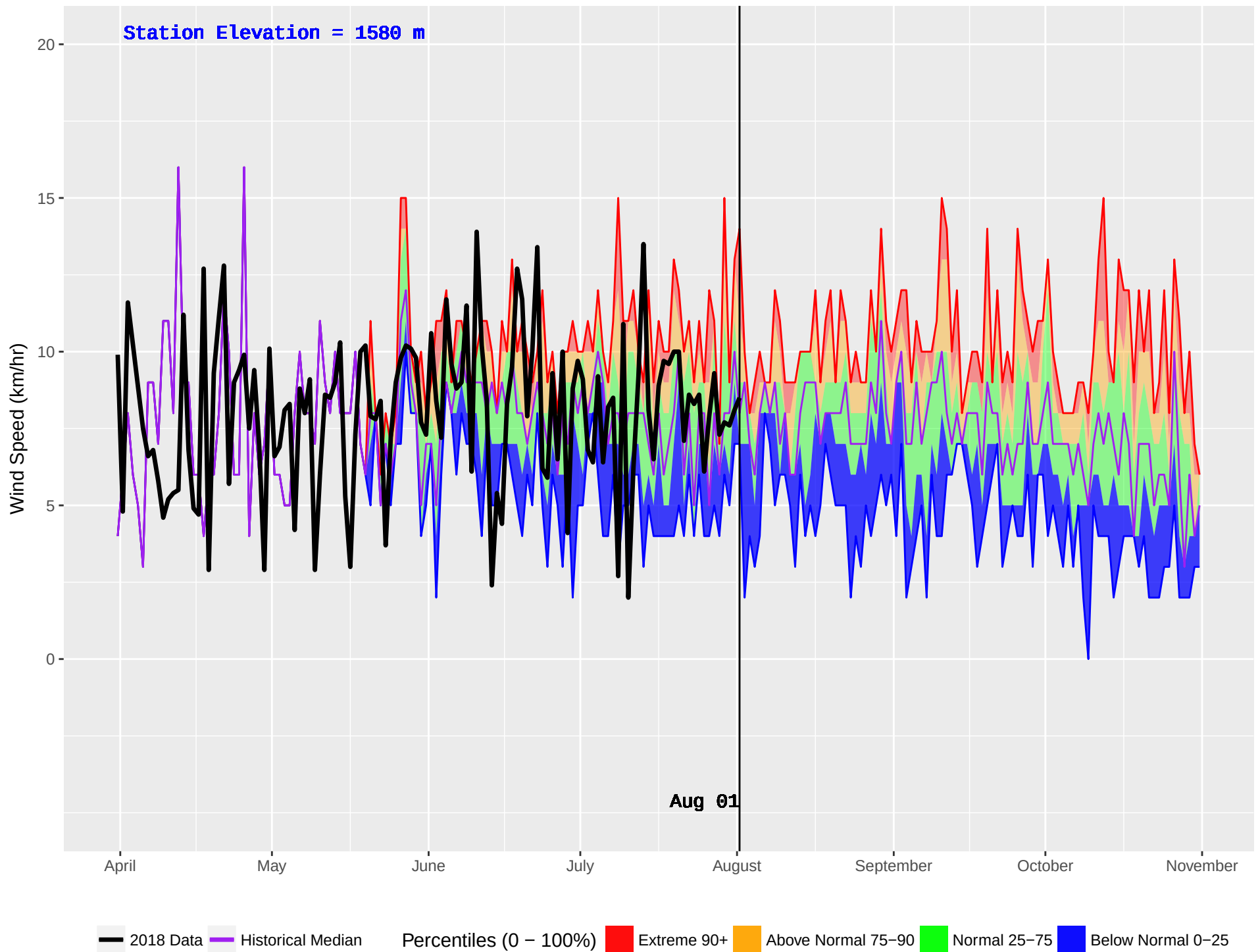
RORY CREEK (1092) : Historical (2010–2016) and Current (2018) Daily Wind Speed
